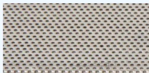
3010 OA 22.7% .0393"t x φ .0295" x .0591" centers
